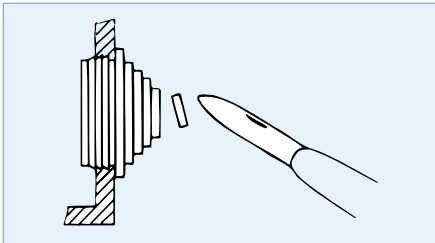
Graduated Diameter, Flexible Cut-to-fit Cable Entries
