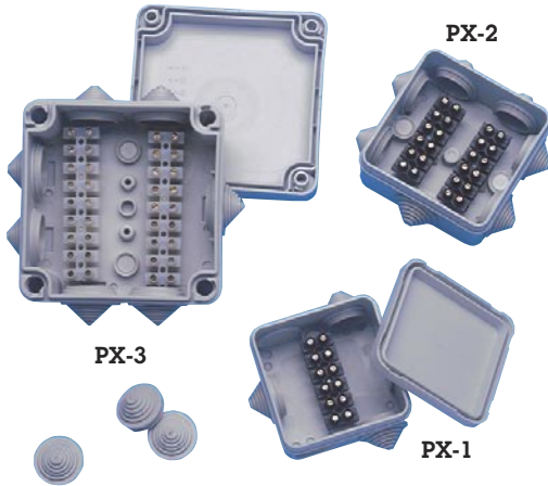
Graduated Diameter, Flexible Cut-to-fit Cable Entries
